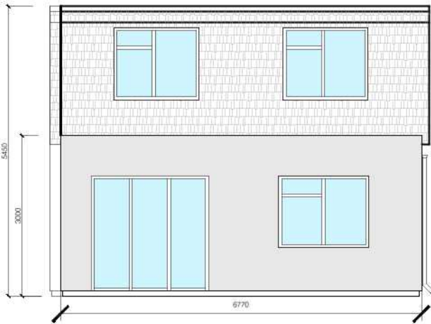
03 1014 Proposed Garden Elevation 1:100@A3
