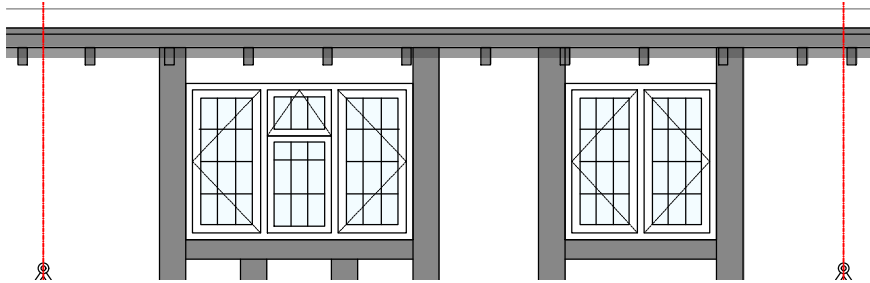
EXISTING WINDOWS - ELEVATION MATERIAL - UPVC
