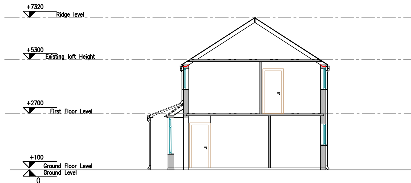
5 EXISTING SECTION (A-A)
