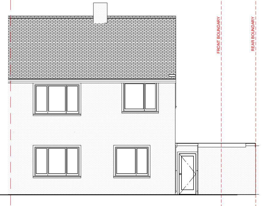
EXISTING REAR (1:100)
