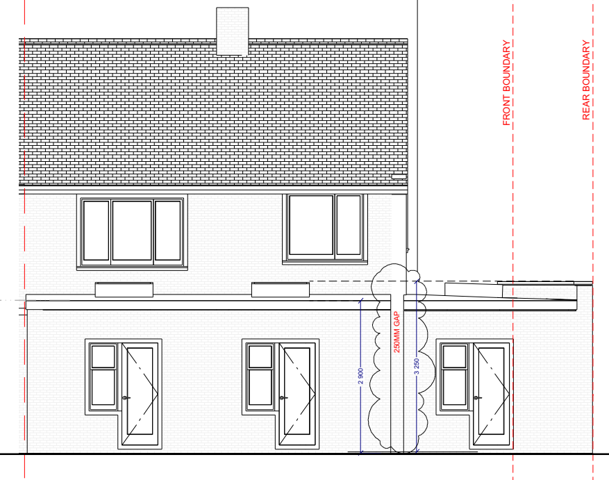
PROPOSED REAR (1:100)
