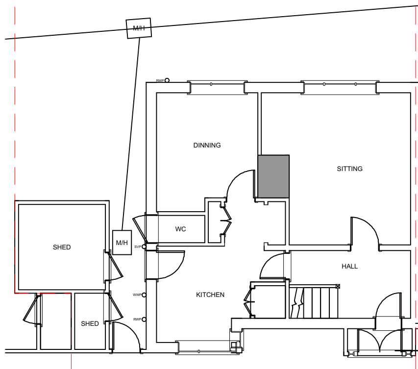
EXISTING G/F (1:100)
