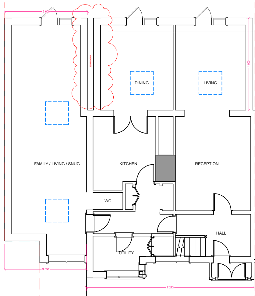
PROPOSED G/F (1:100)
