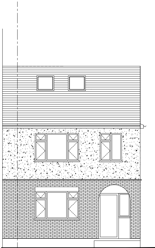
Front Elevation
