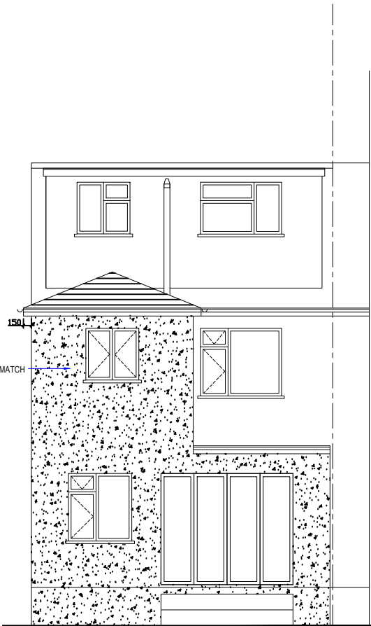
Rear Elevation
