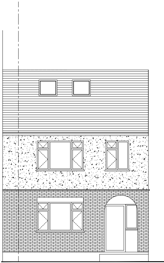
Front Elevation
