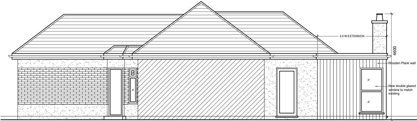
03 - RIGHT SIDE ELEVATION
