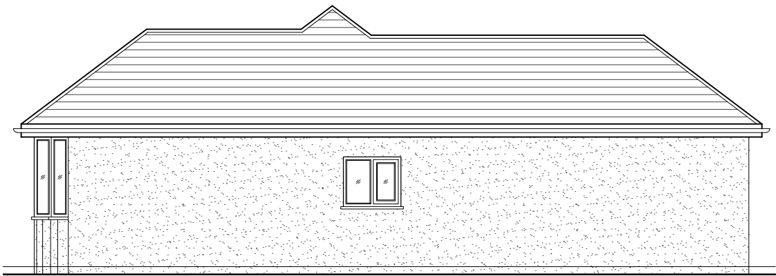
04 - LEFT SIDE ELEVATION
