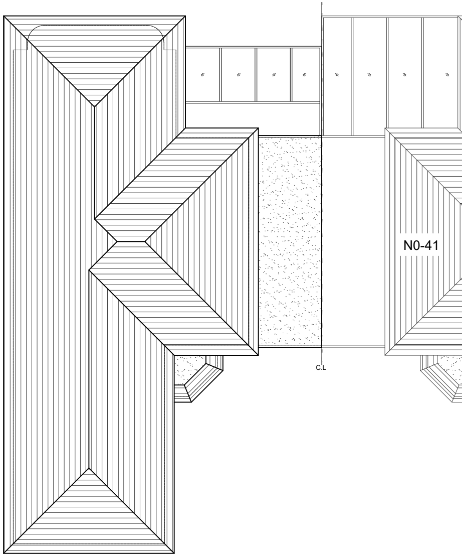
02 - ROOF PLAN
