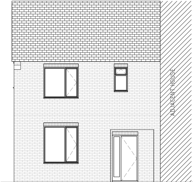
04/201 - EXISTING FRONT ELEVATION 1: 100
