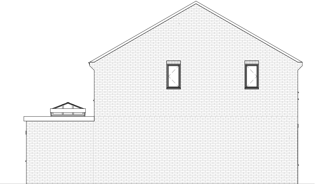
04/202 - EXISTING LEFT ELEVATION 1: 100
