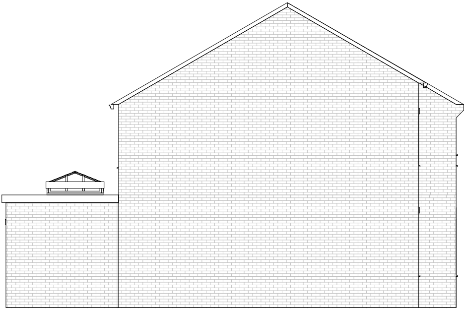
06/402 – PROPOSED LEFT ELEVATION 1 : 100
