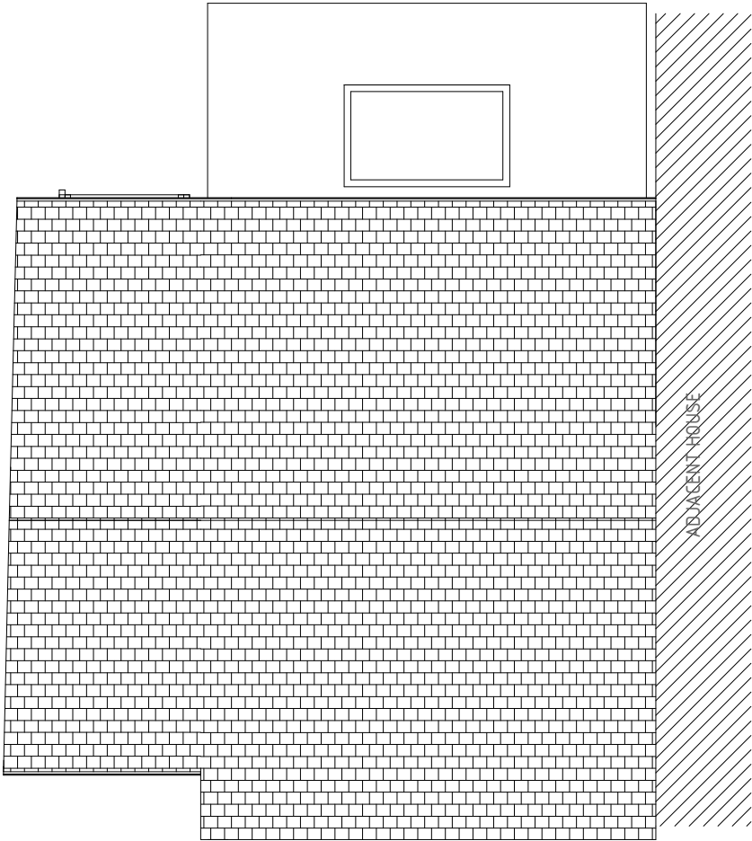
05/304 – PROPOSED ROOF PLAN 1: 100
