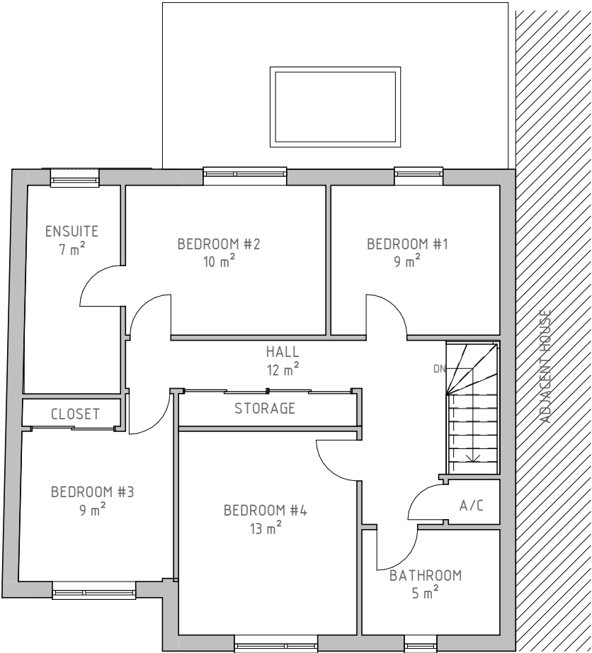
05/302 – PROPOSED FIRST FLOOR PLAN 1: 100
