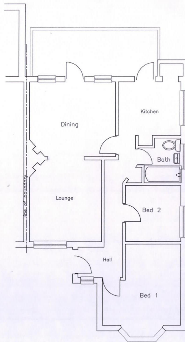
Ground floor plan extg 1:100
