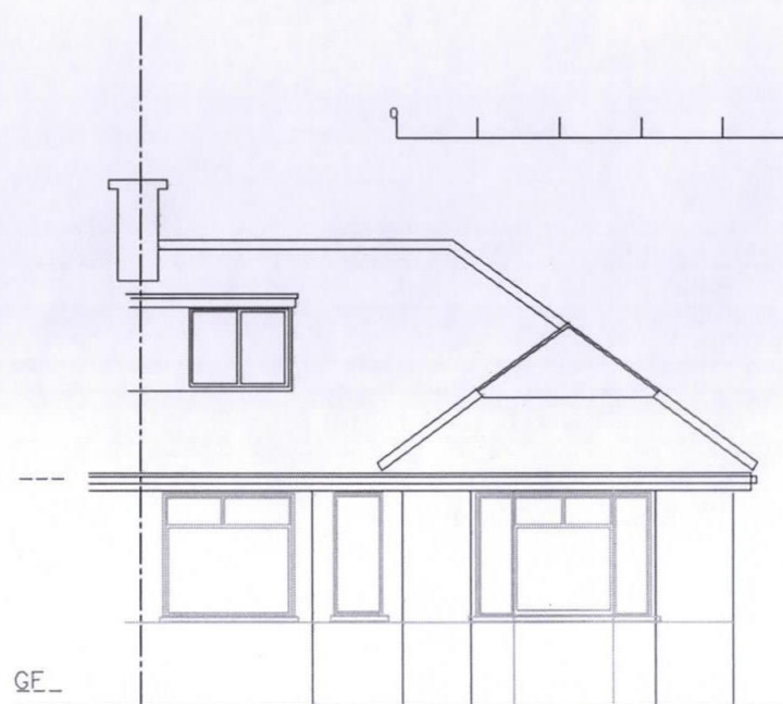
Front Elevation 1:100
