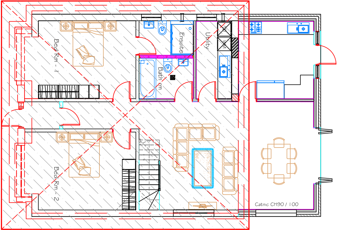
Proposed Demolition - Demolish Front Bays EXISTING GROUND FLOOR PLAN
