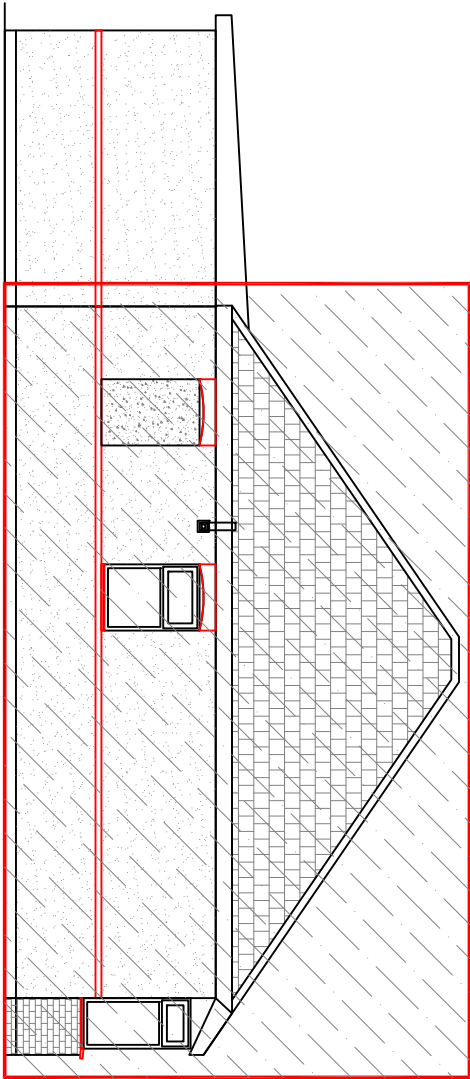
Proposed Demolition - Demolish Entire Roof
