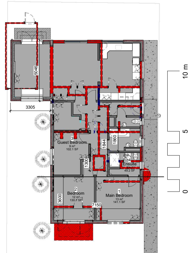
3 Proposed and Demo 1 : 100
