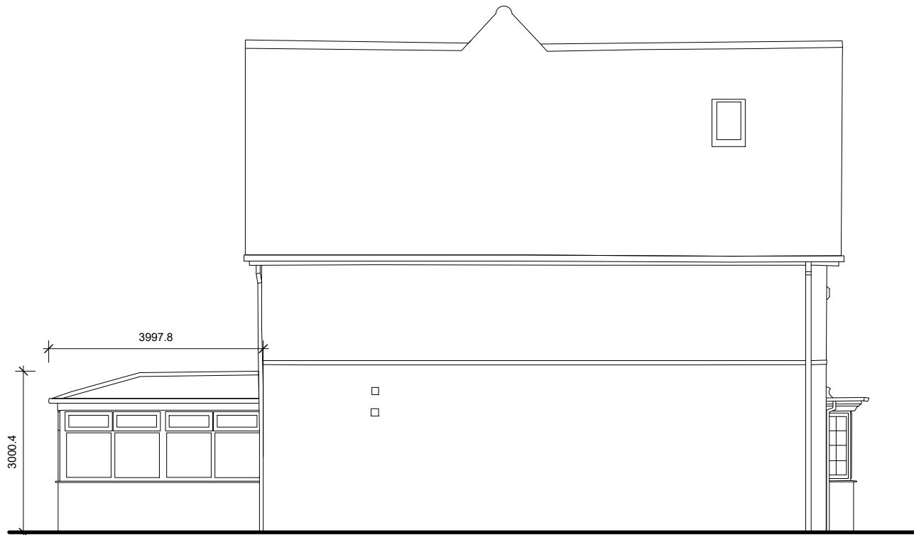
2 EXISTING NORTH SIDE ELEVATION 1 : 100
