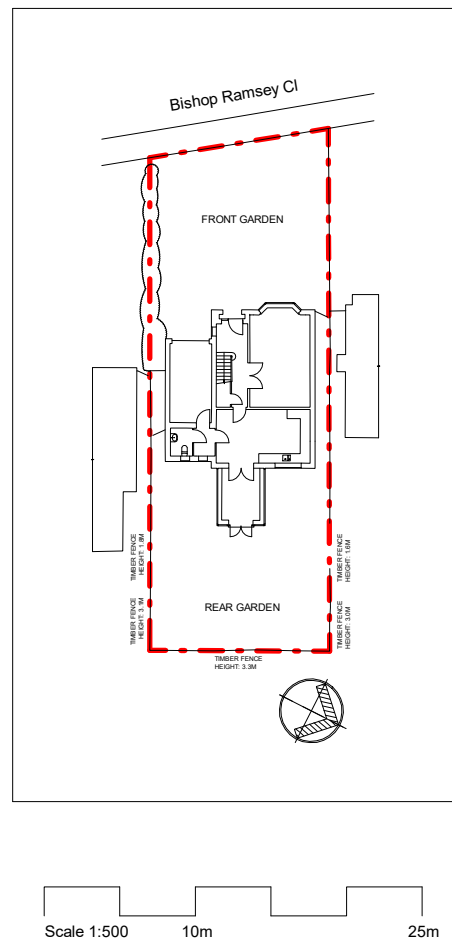
2 Existing Block Plan 1 : 500
