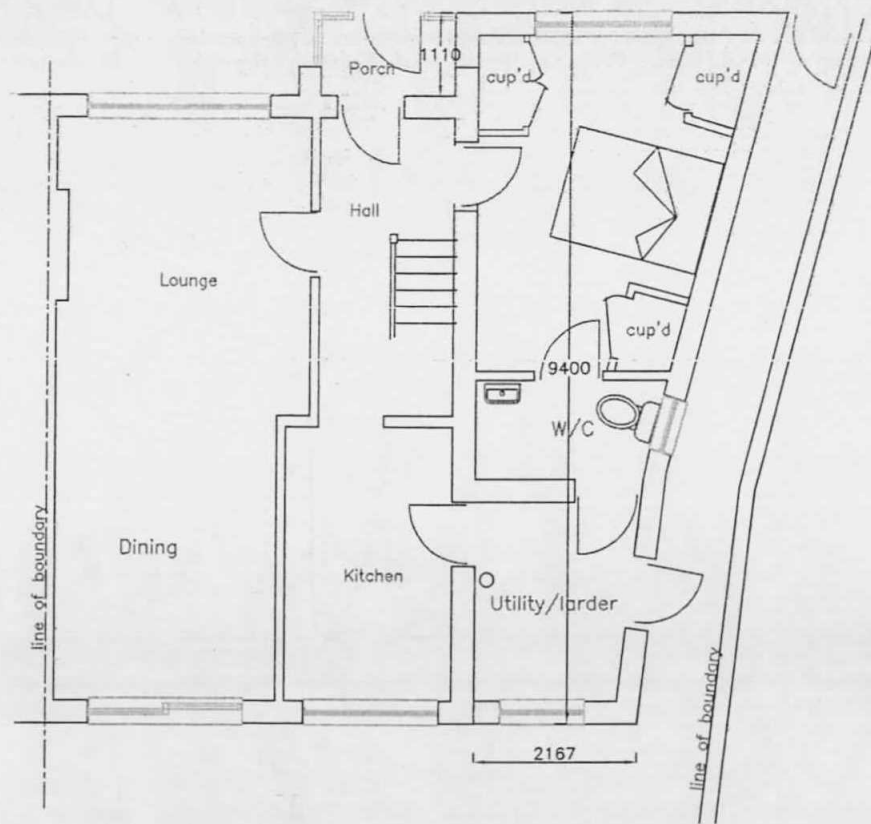
Ground floor plan proposed 1:100
