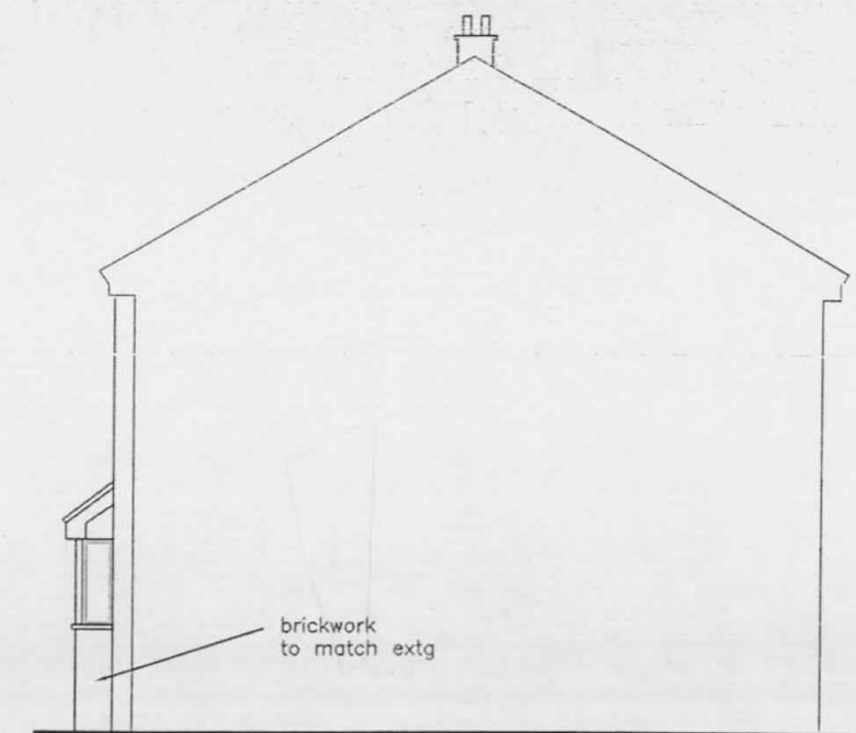
Side Elevation 1:100
