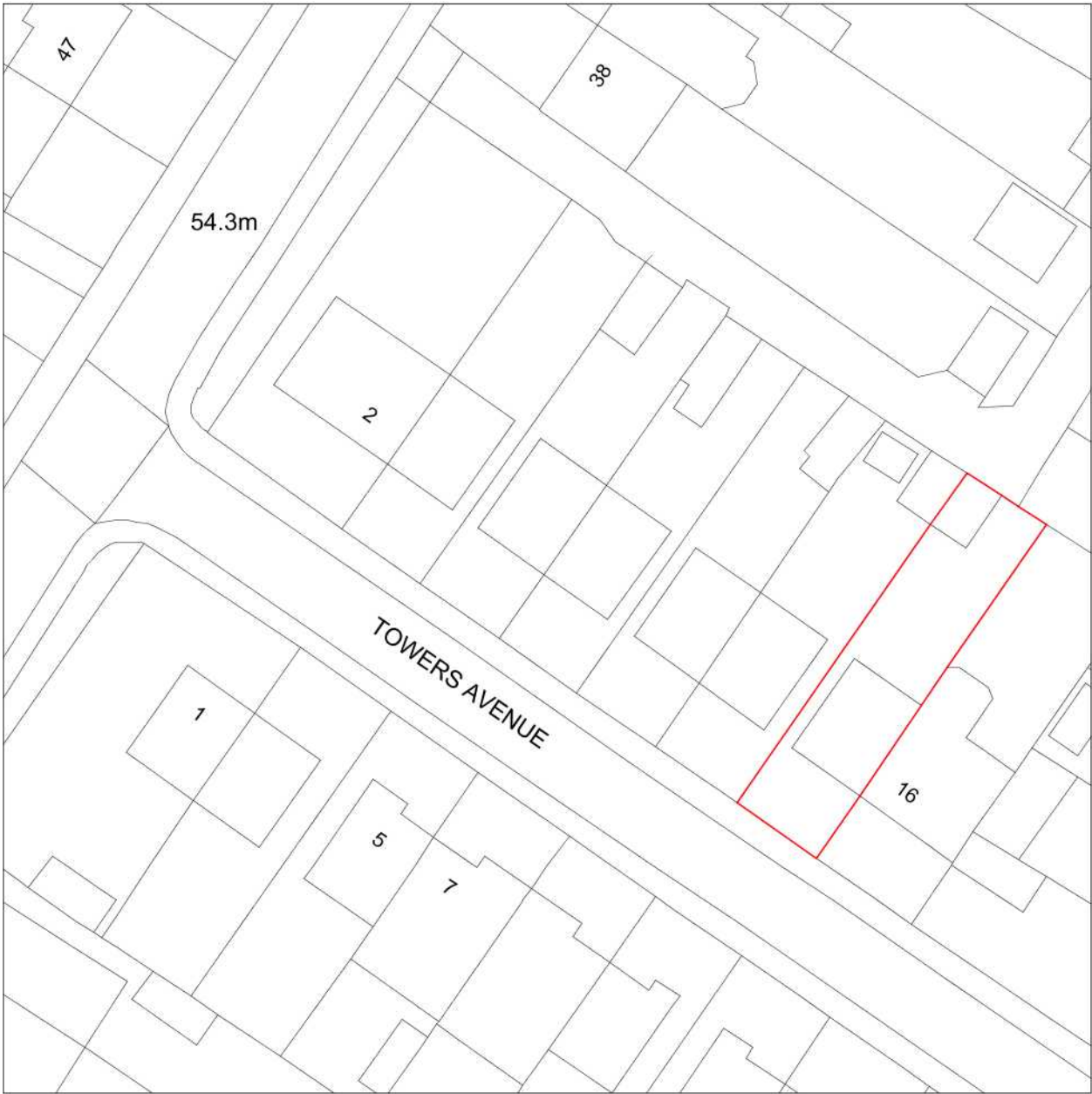
Block Plan 1:500
