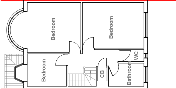
Existing First Floor Plan Scale 1:100
