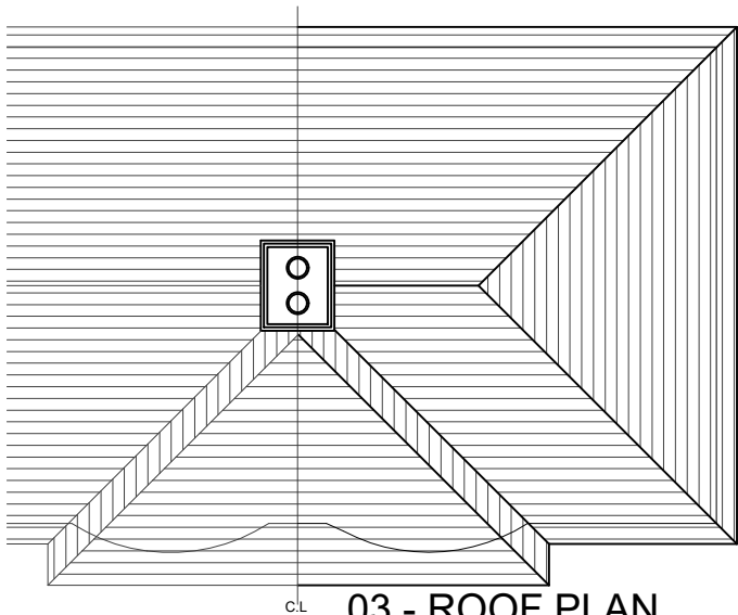
03 - ROOF PLAN
