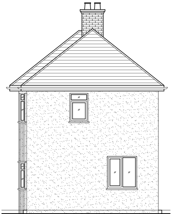
06 - SIDE ELEVATION
