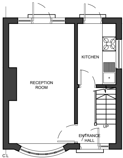
01 - GROUND FLOOR PLAN
