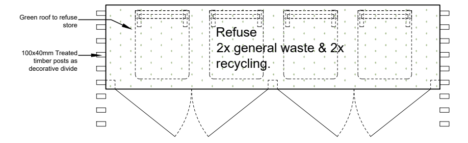
Refuse Stores 2x 240 ltr general waste wheelie bin, 2x 240 ltr dry recycling wheelie bin scale 1:20@A1 (1:40@A3)
