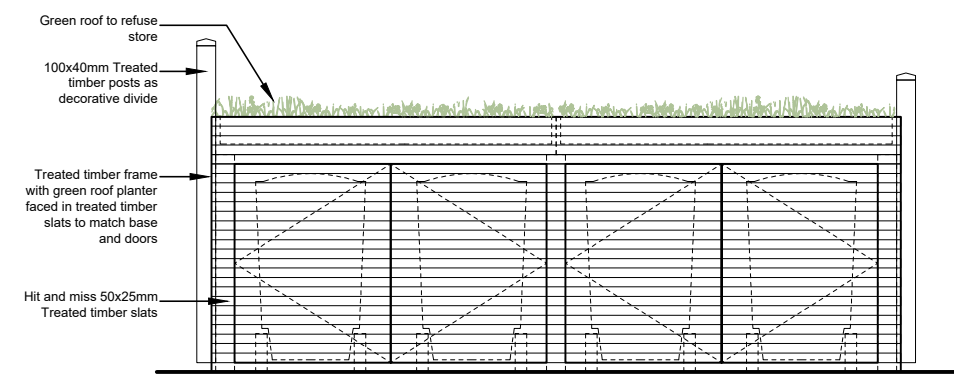
Refuse Stores 2x 240 ltr general waste wheelie bin, 2x 240 ltr dry recycling wheelie bin scale 1:20@A1 (1:40@A3)
