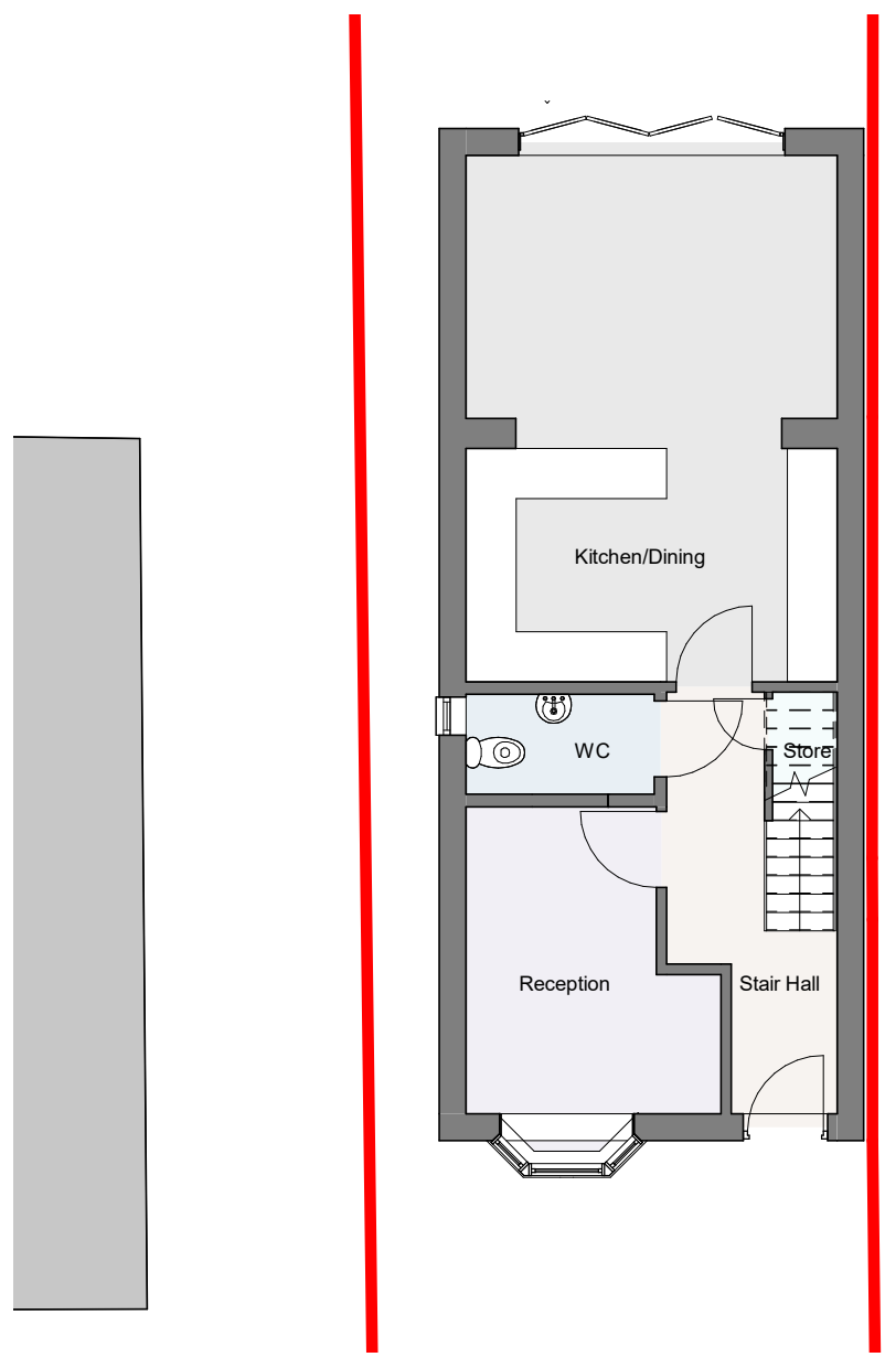
1 Proposed Ground Floor Plan 2318-VA-200 1 : 100
