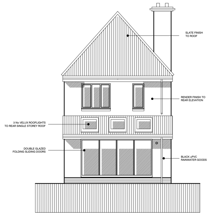
REAR ELEVATION TO GARDEN
