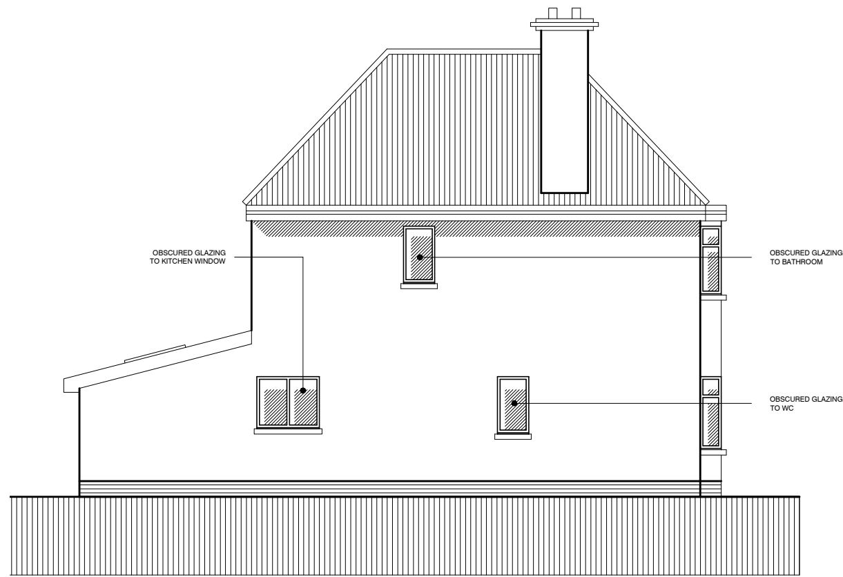
SIDE ELEVATION
