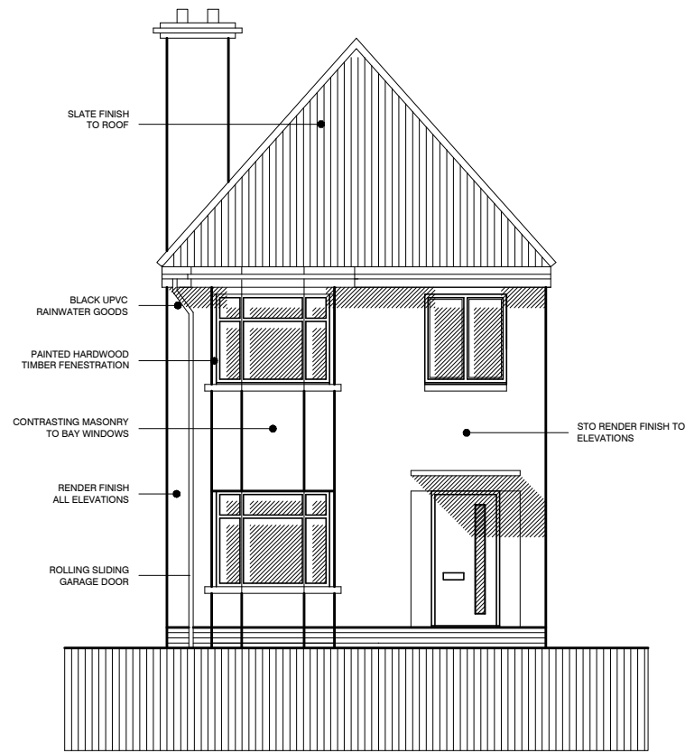
FRONT ELEVATION
