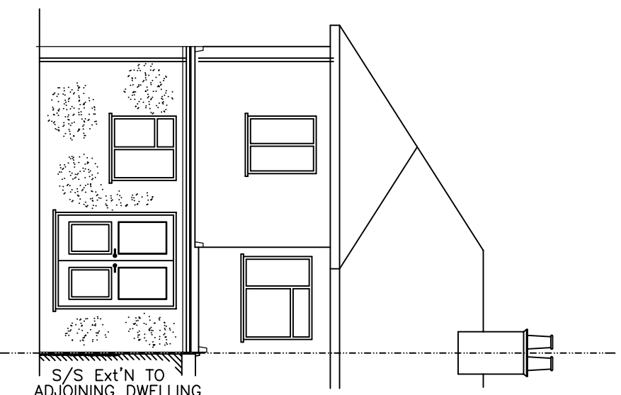
REAR ELEVATION
