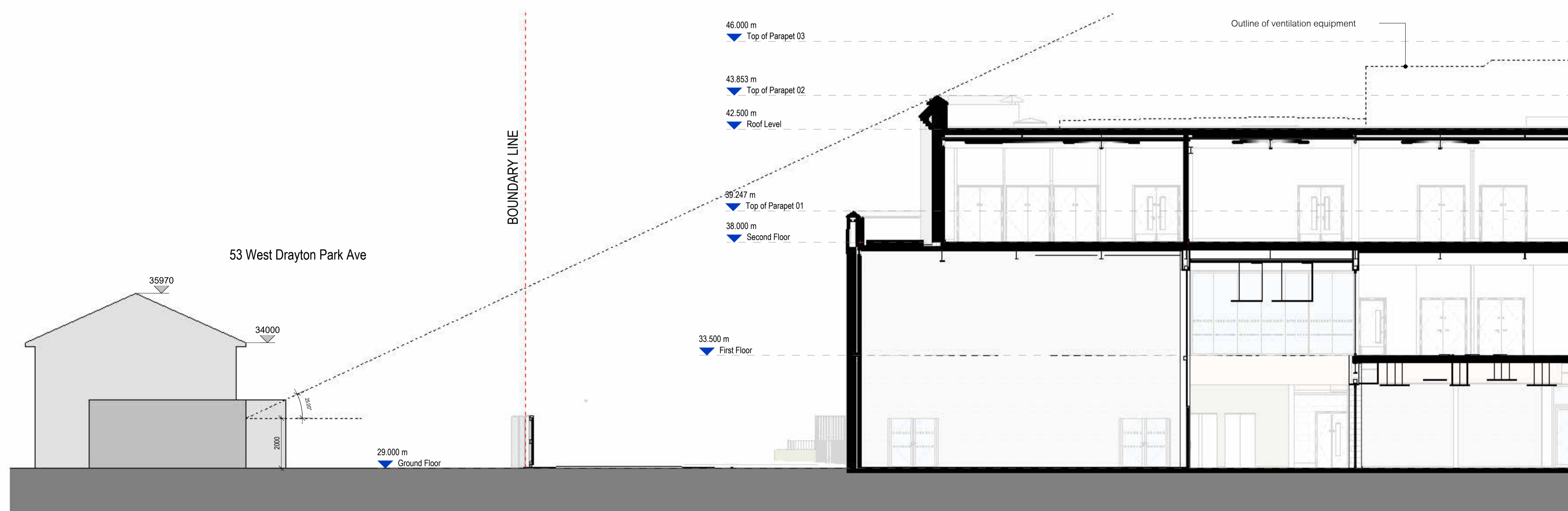
2 Section at no. 53 1 : 100
