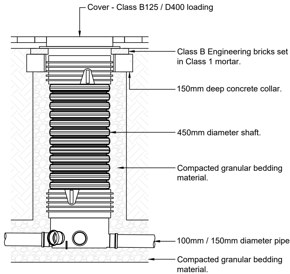
450mm PPIC - B125 / D400 Cover (Scale 1:20)
