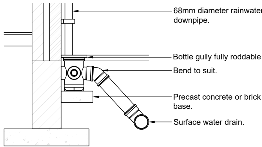
RWP to Bottle Gully - Section (Scale 1:20)
