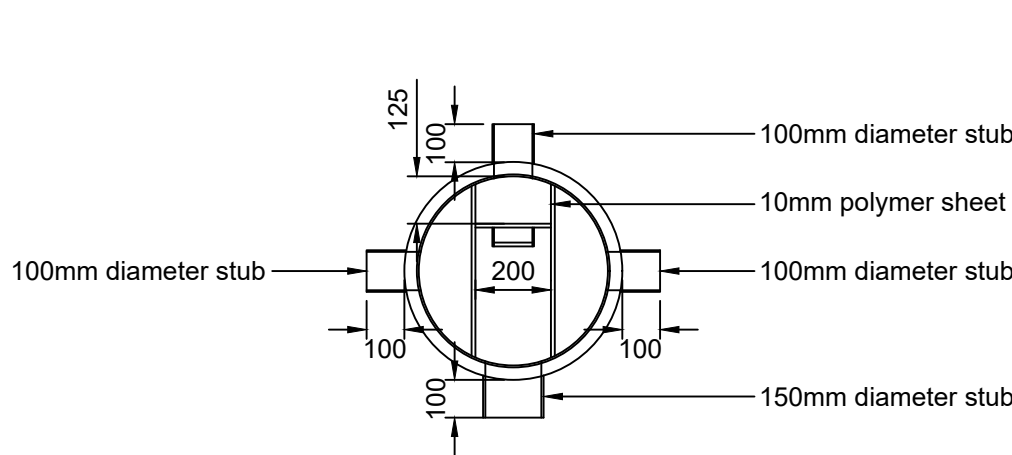
Orifice Flow Control Chamber - Plan (Scale 1:20)
