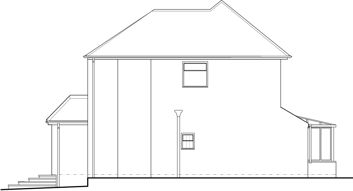
Proposed North East Elevation Scale 1:100
