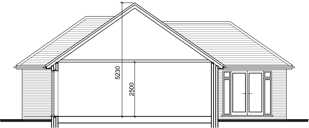
Typical Section Scale - 1:100
