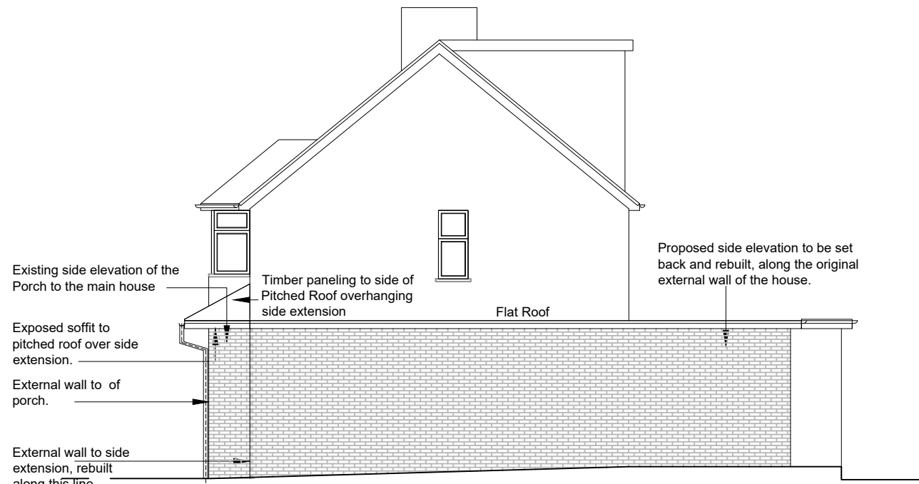
Side extension Facing Nos. 4 Side Elevation looking from Nos 4 Showing Proposed Side Extension- Sc 1:100
