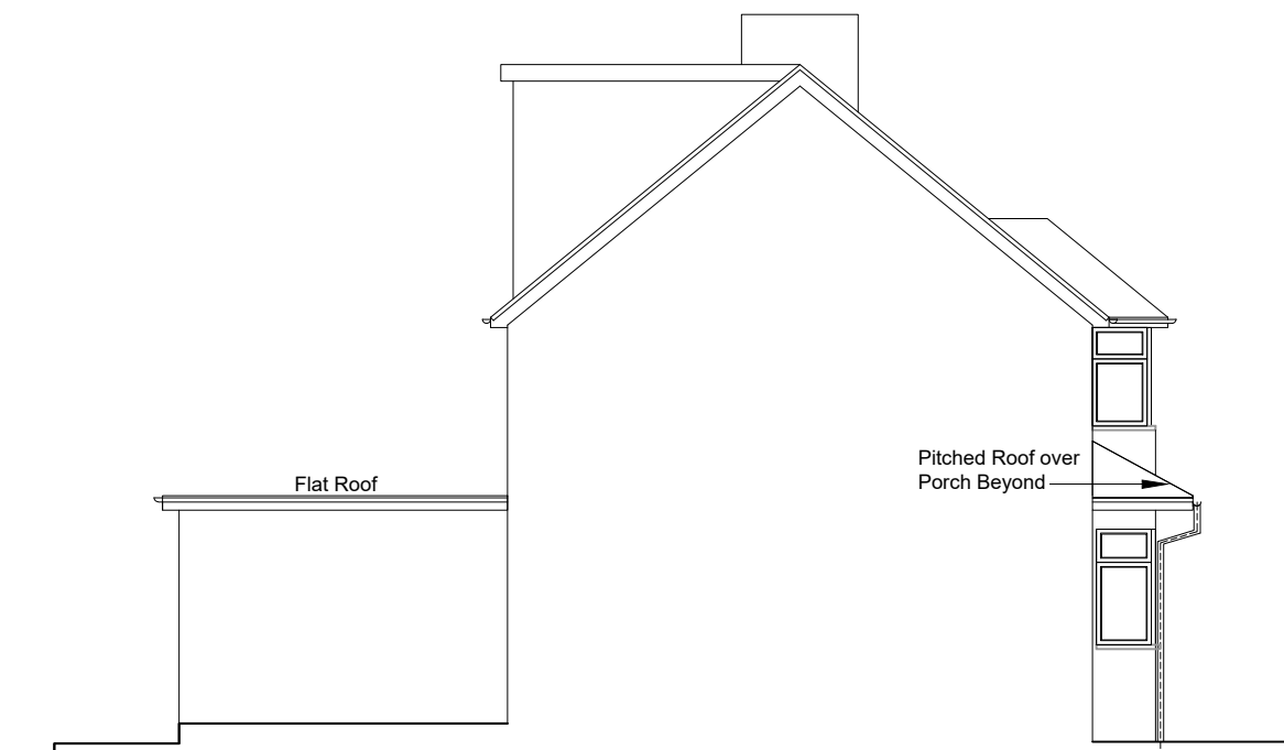
Side Elevation looking from No 8 Showing Proposed Side Extension- Sc 1:100
