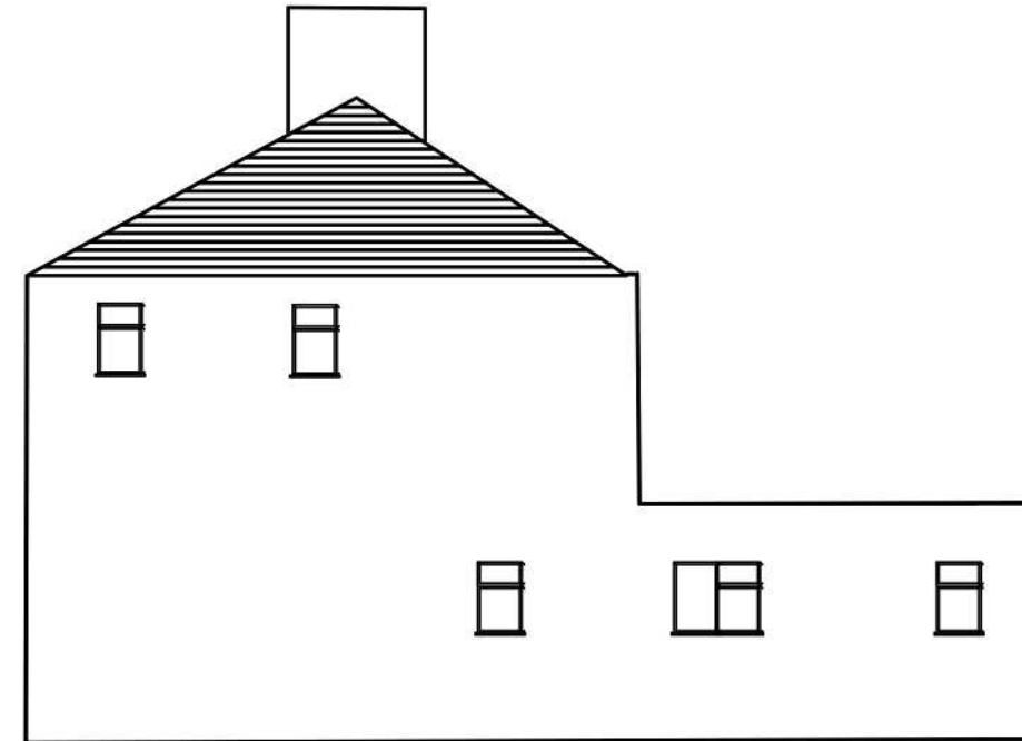
Proposed Right Side Elevation 1:100
