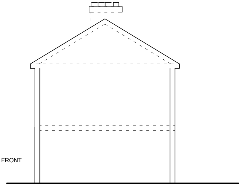
EXISTING SIDE ELEVATION (VIEW FROM NO. 58 SIDE)
