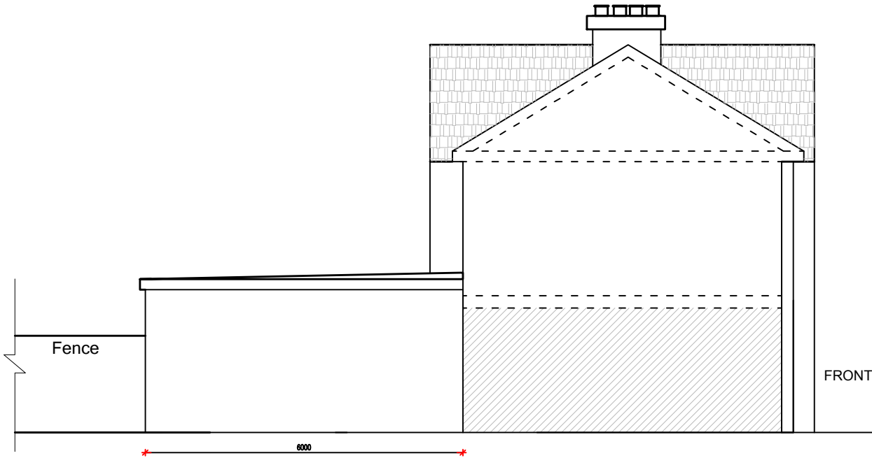
PROPOSED SIDE ELEVATION (VIEW A)
