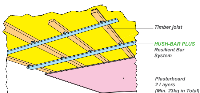
HUSH-BAR PLUS RESILIENT BAR SYSTEM
