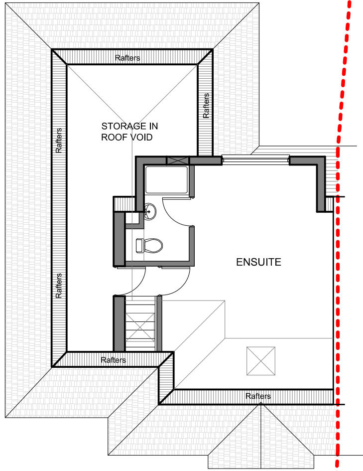
PROPOSED LOFT FLOOR PLAN
