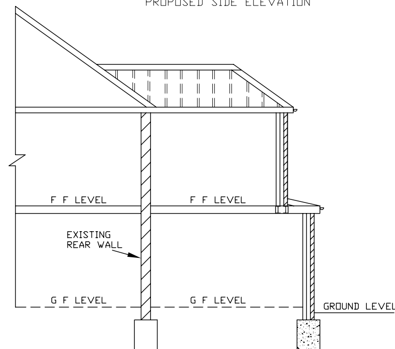
SECTION THROUGH THE EXTENSION
