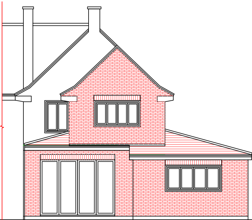
PROPOSED REAR PARTY-SIDE ELEVATION
