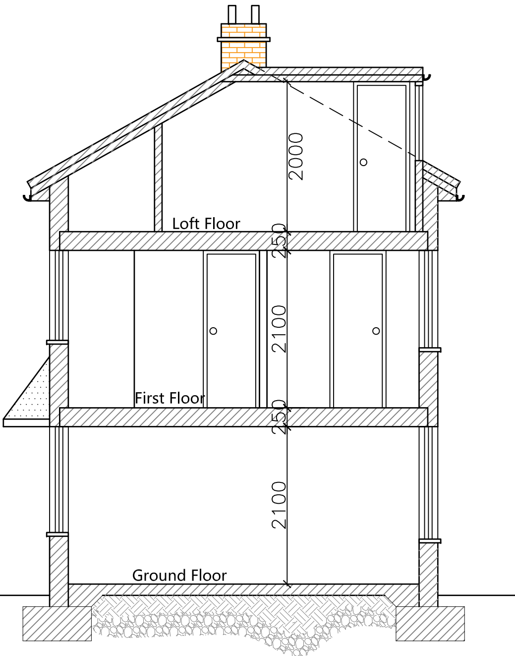
Proposed Section
