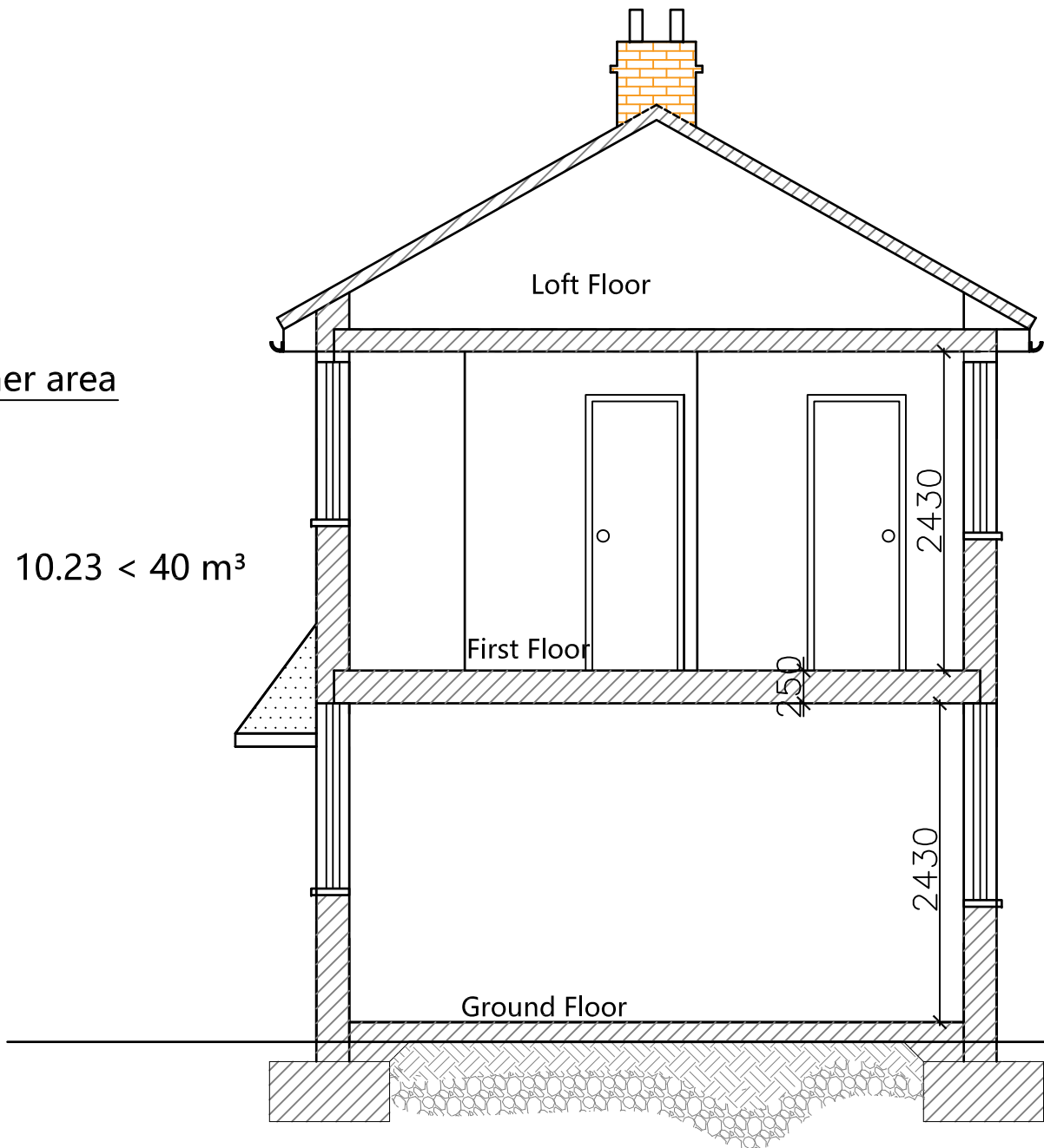
Existing Section
