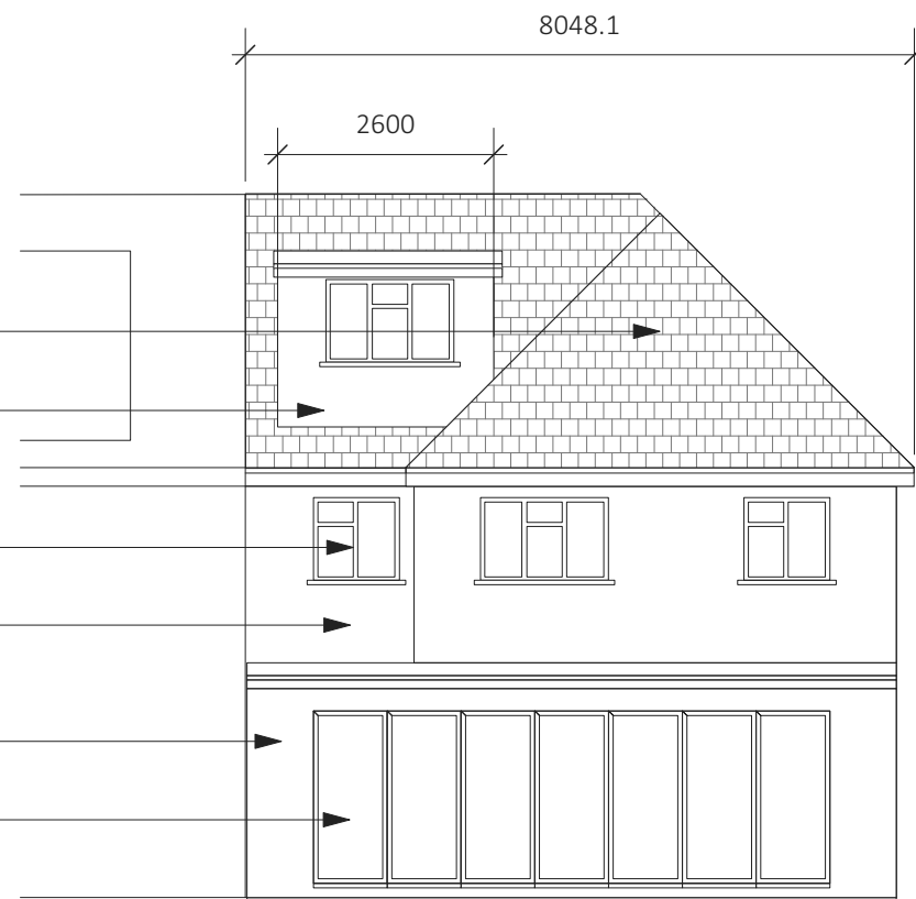
Rear elevation
