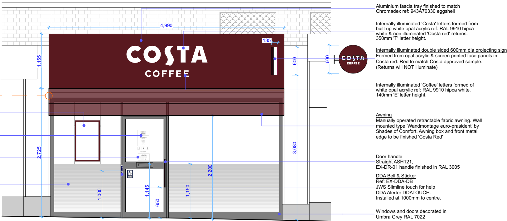
Proposed Shopfront 1:50
