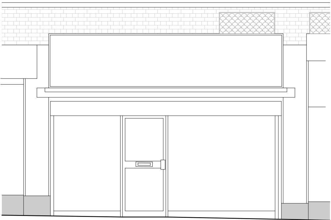
Existing Shopfront 1:50
