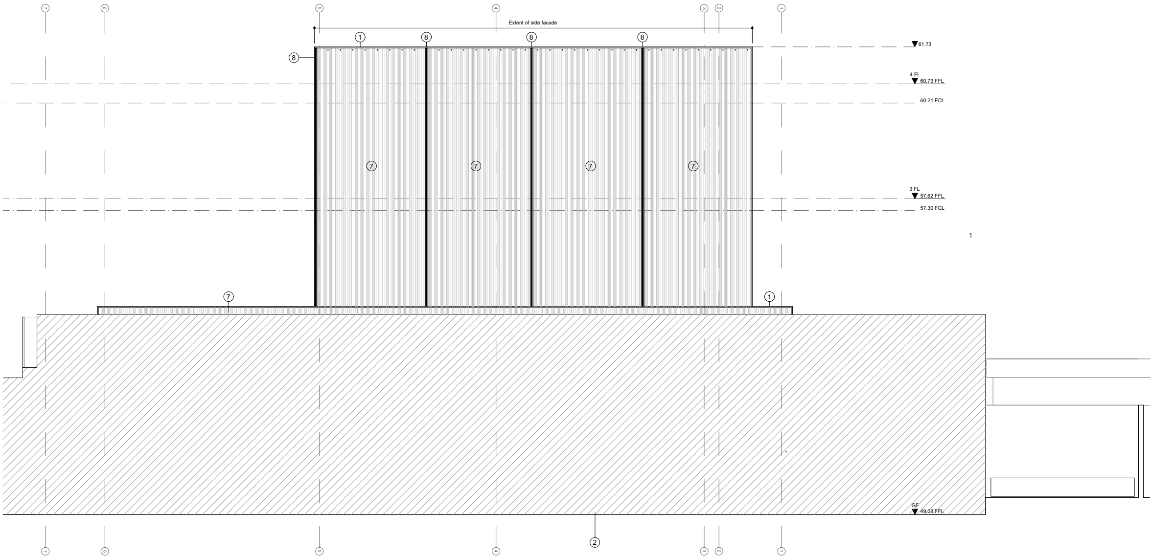
01 Side Elevation- 1:100
