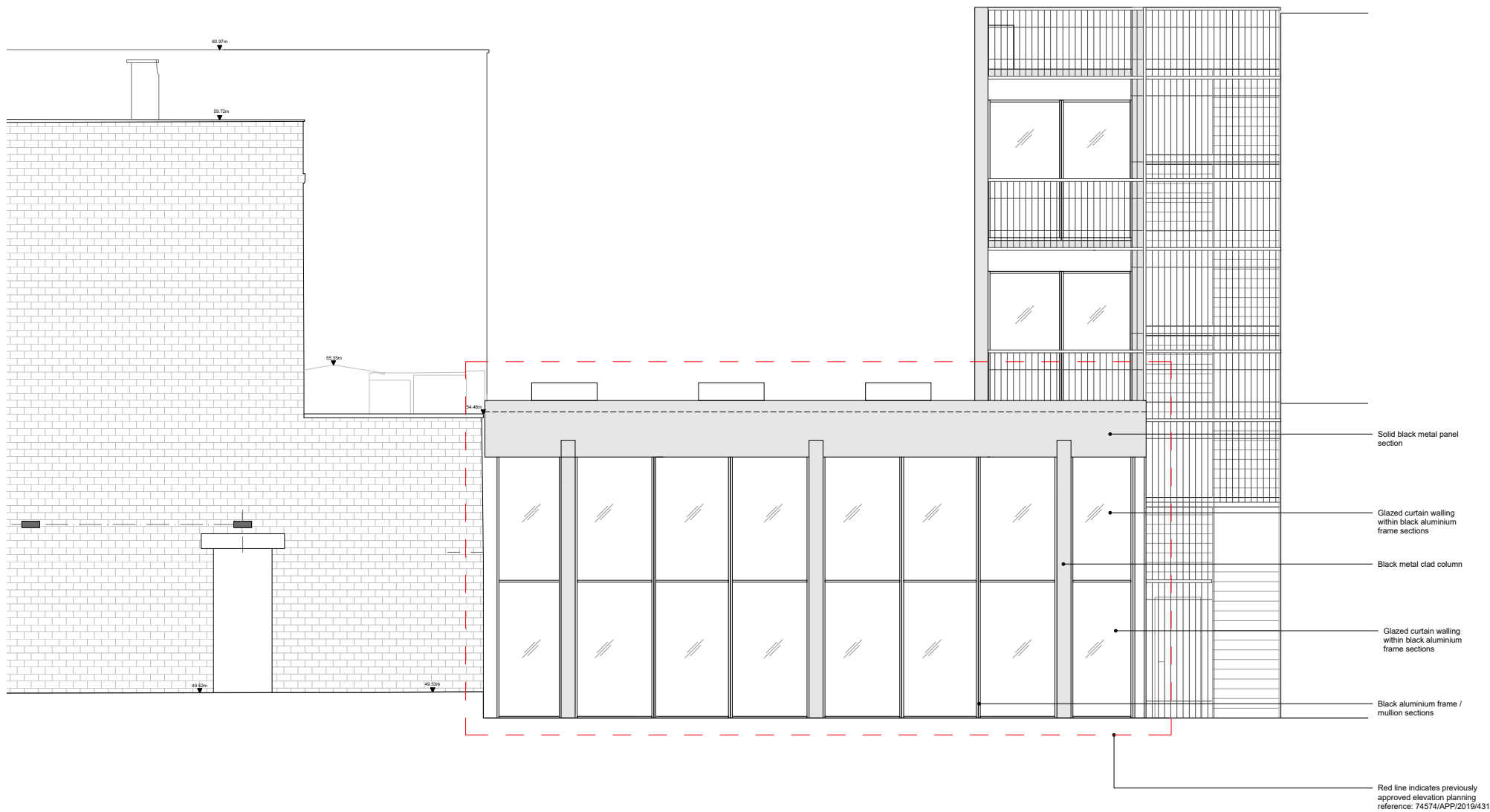
01 PLANNING APPROVED FRONT ELEVATION 1:100 REF NO. 74574/APP/2019/431
