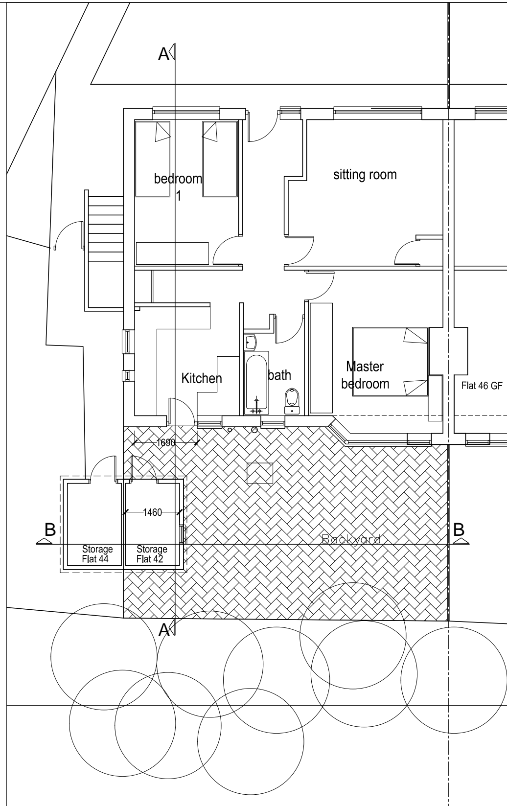
GF plan (Existing)
