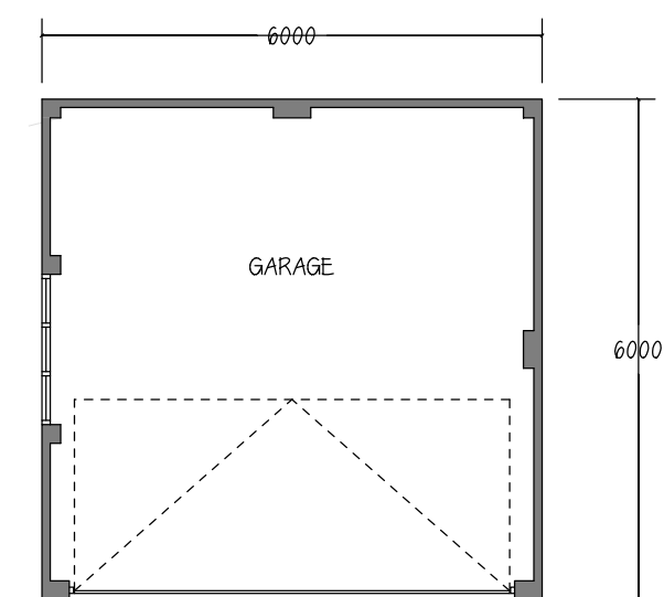
1:100 FLOOR PLAN
