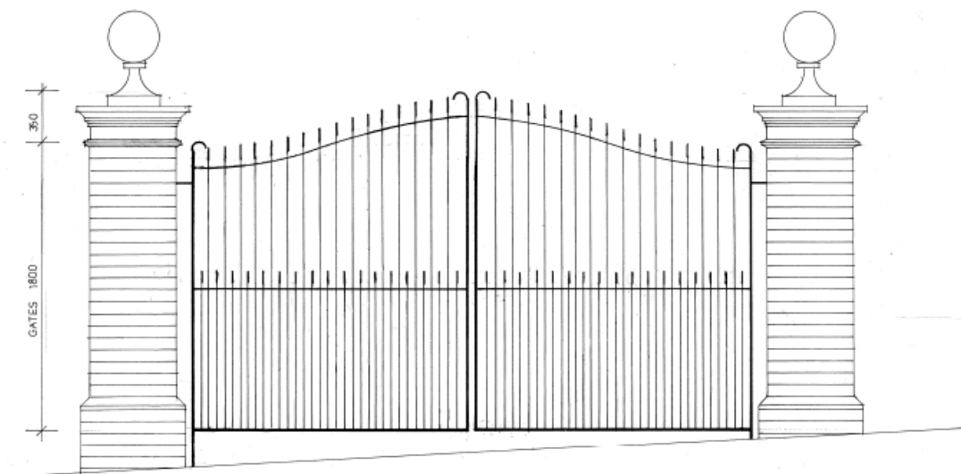
GATES AND PIERS ELEVATION
