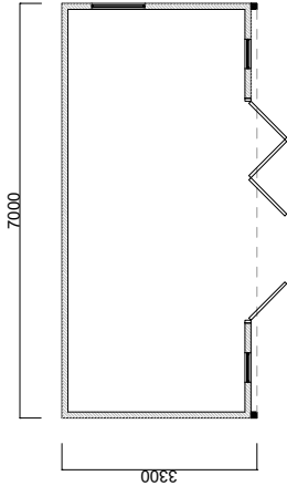
Proposed Ground Floor Plan
