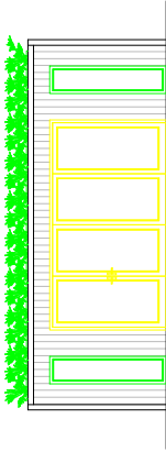
Proposed Front Elevation
