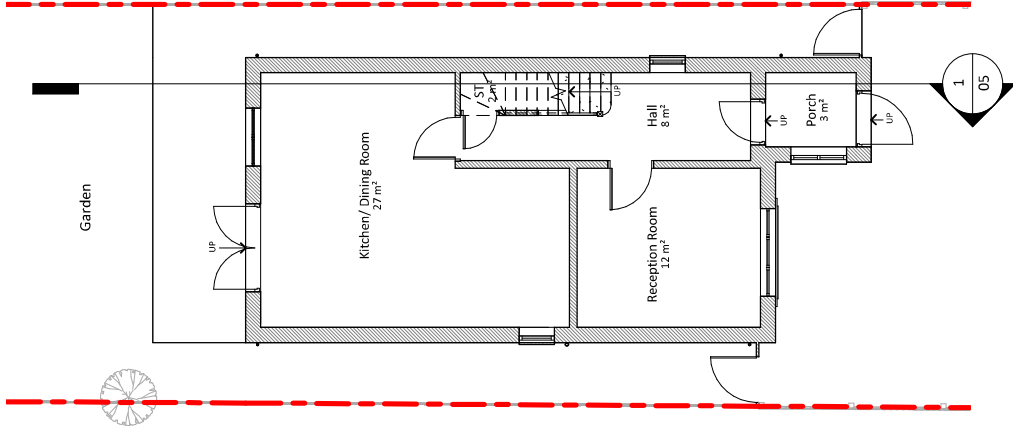
1 Ground Floor Plan
