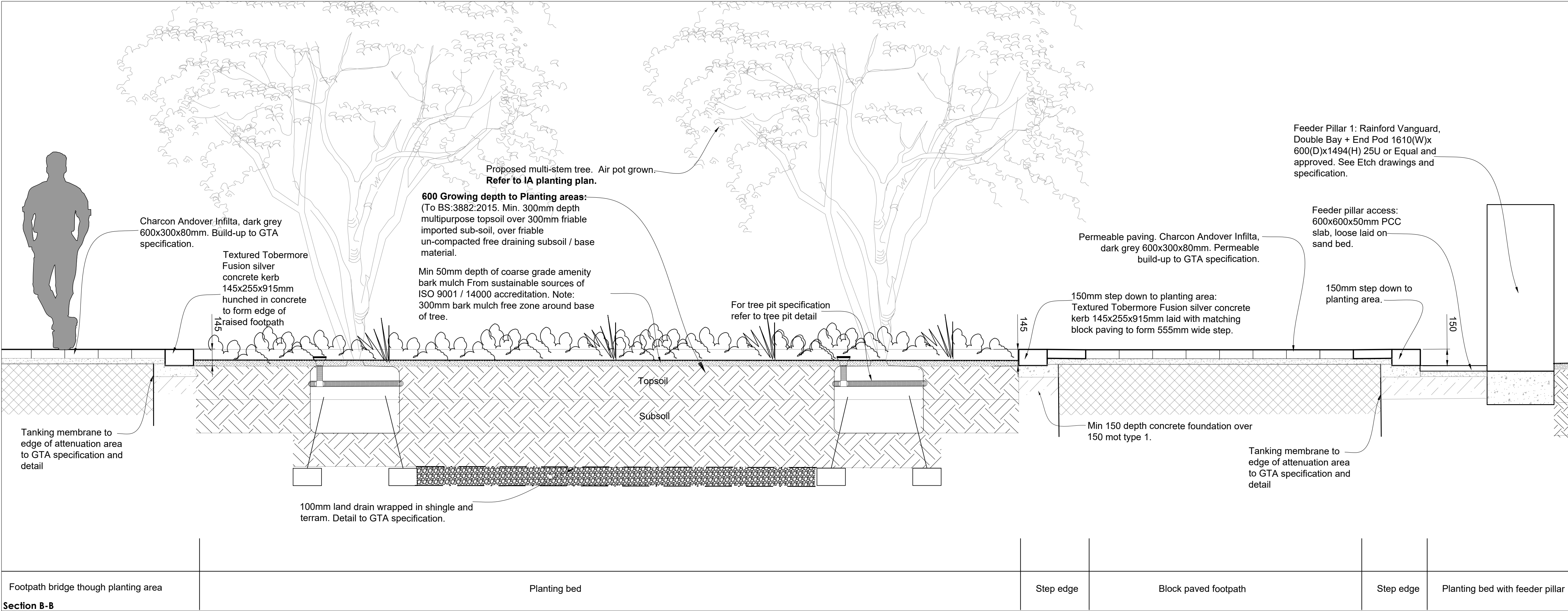
Section B-B Scale 1:20@A1
