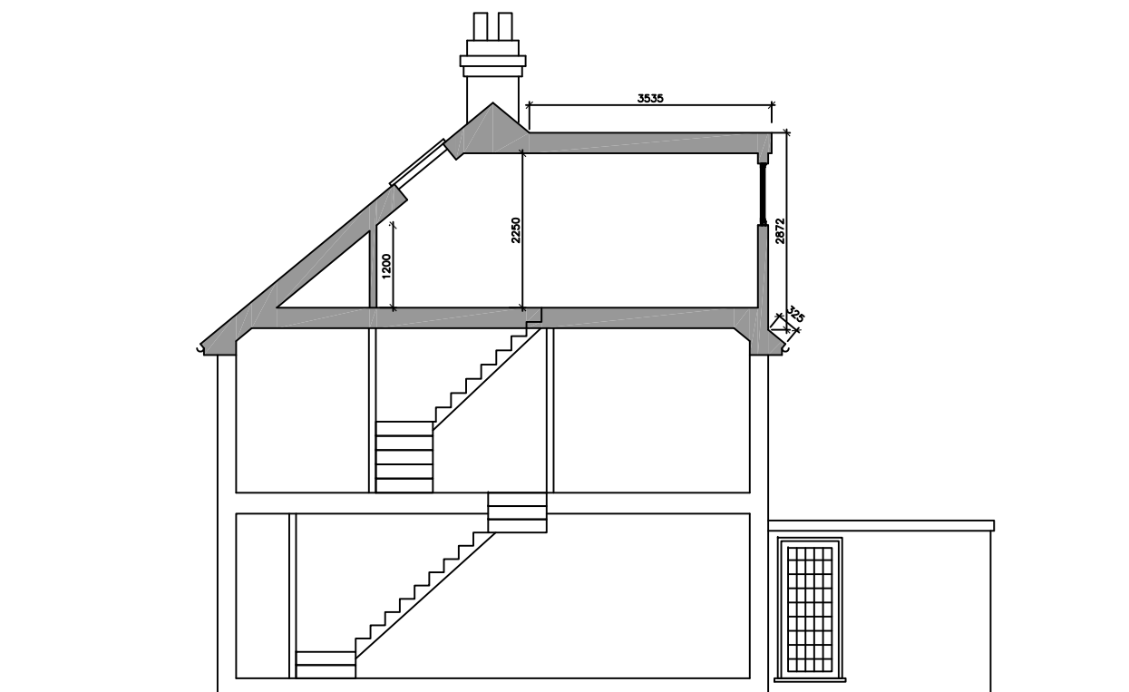
PROPOSED SECTIONAL SIDE ELEVATION
