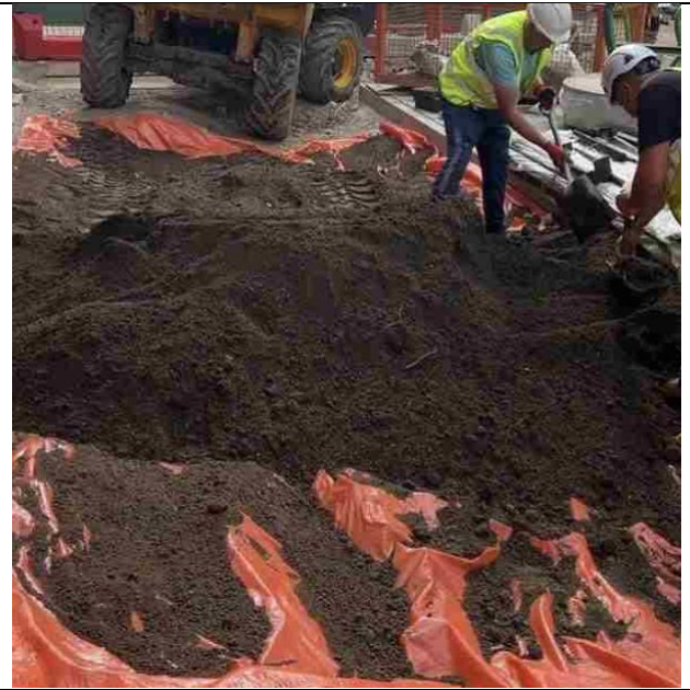
Example of marker layer laying and lapping with concrete (Blocks A and D)
