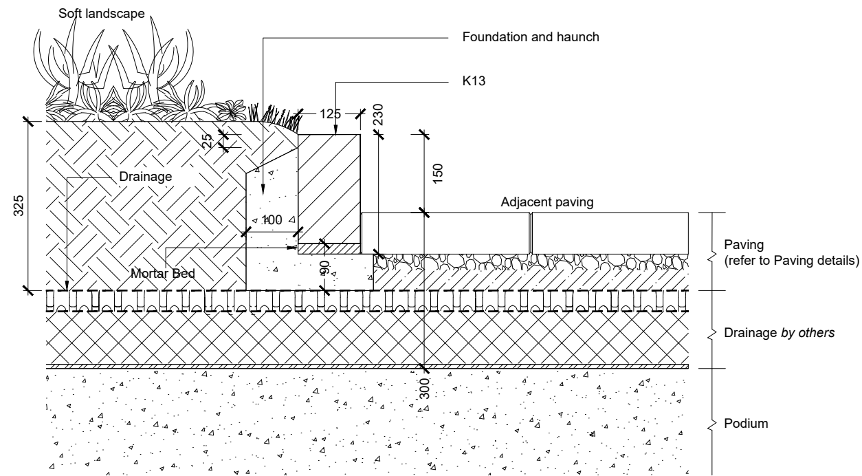
13 2061 PODIUM: RAISED KERB (125mm upstand)
