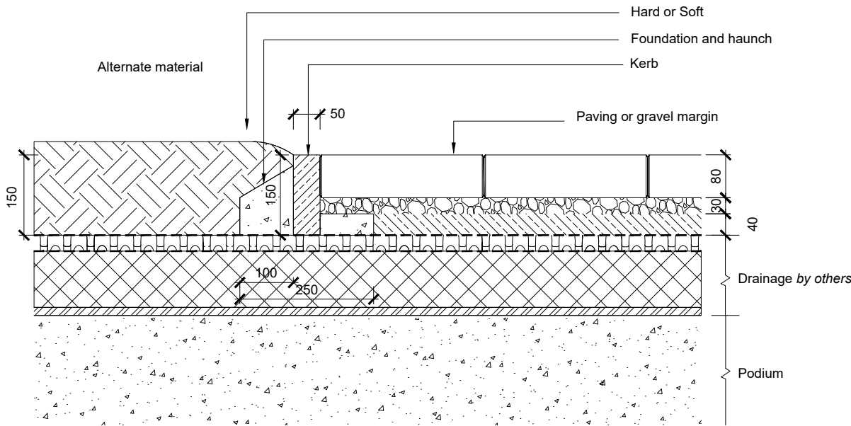
14 2061 PODIUM: FLUSH KERB
