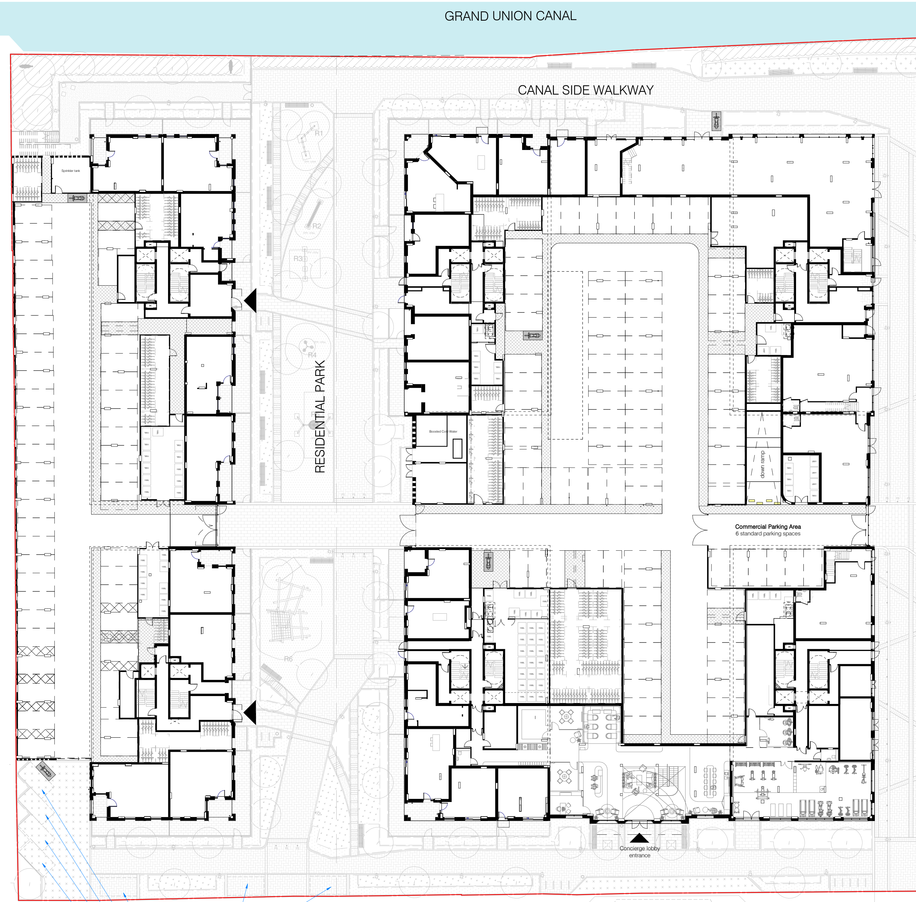
Ground Floor 1 : 300
